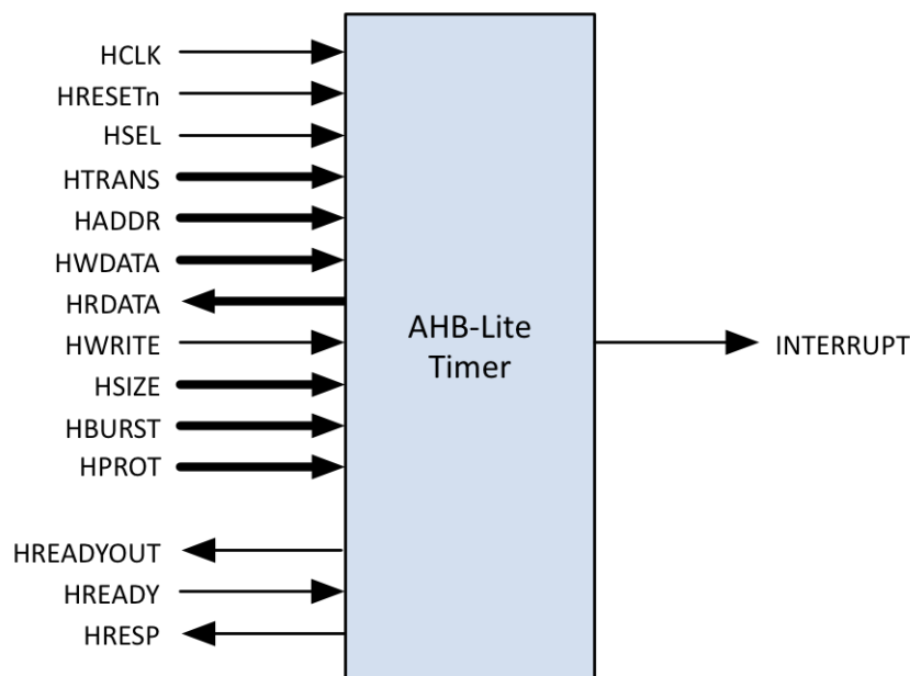
Figure 1.1: AHB-Lite Timer
